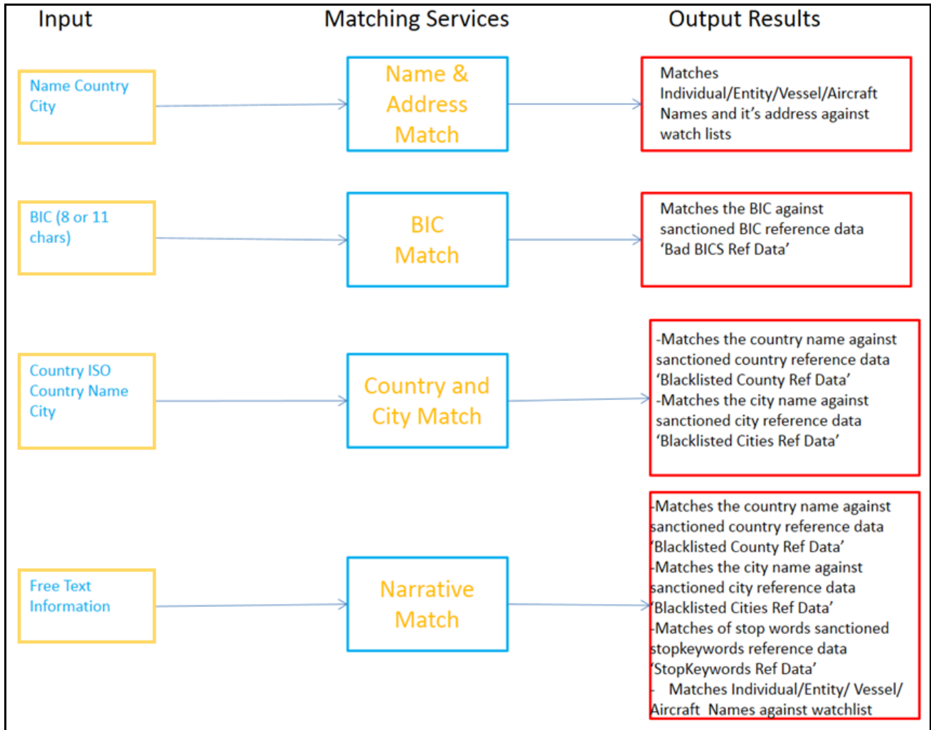
Figure 1. Matching Webservices
